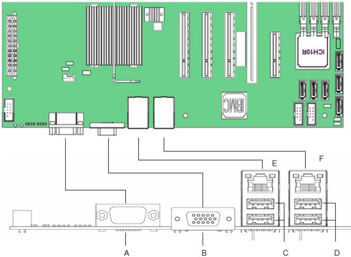
Figure 11. External I/O Layout
