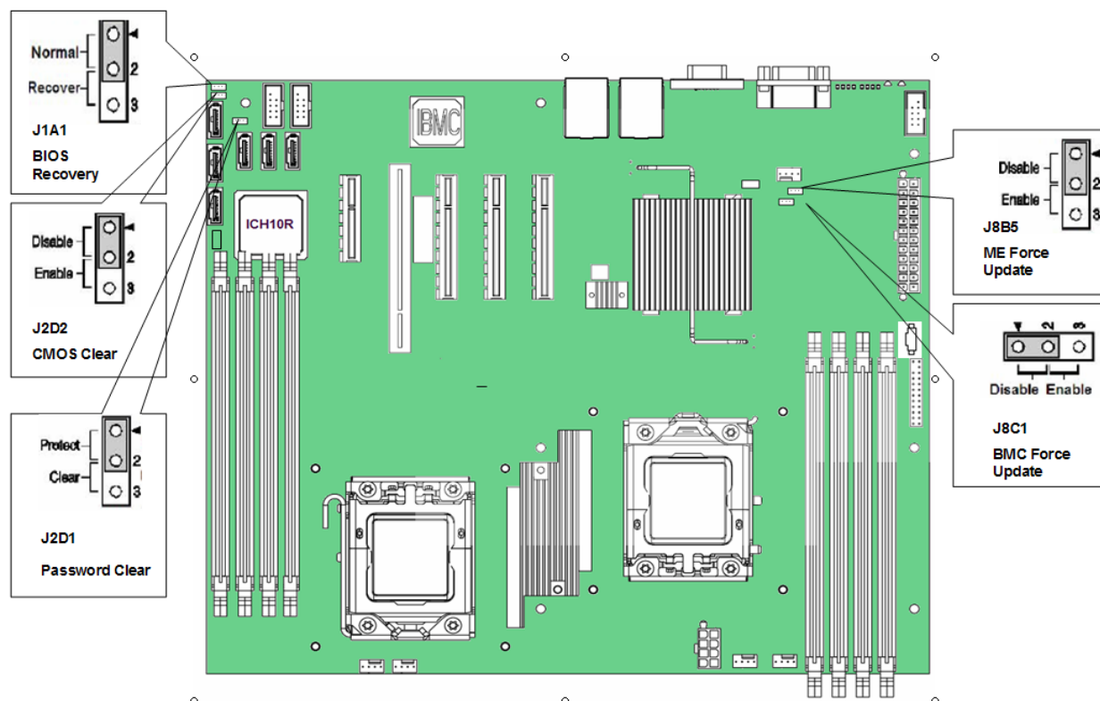
Figure 44. Jumper Blocks
