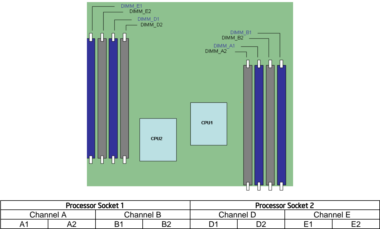
Figure 15. DIMM Organization
