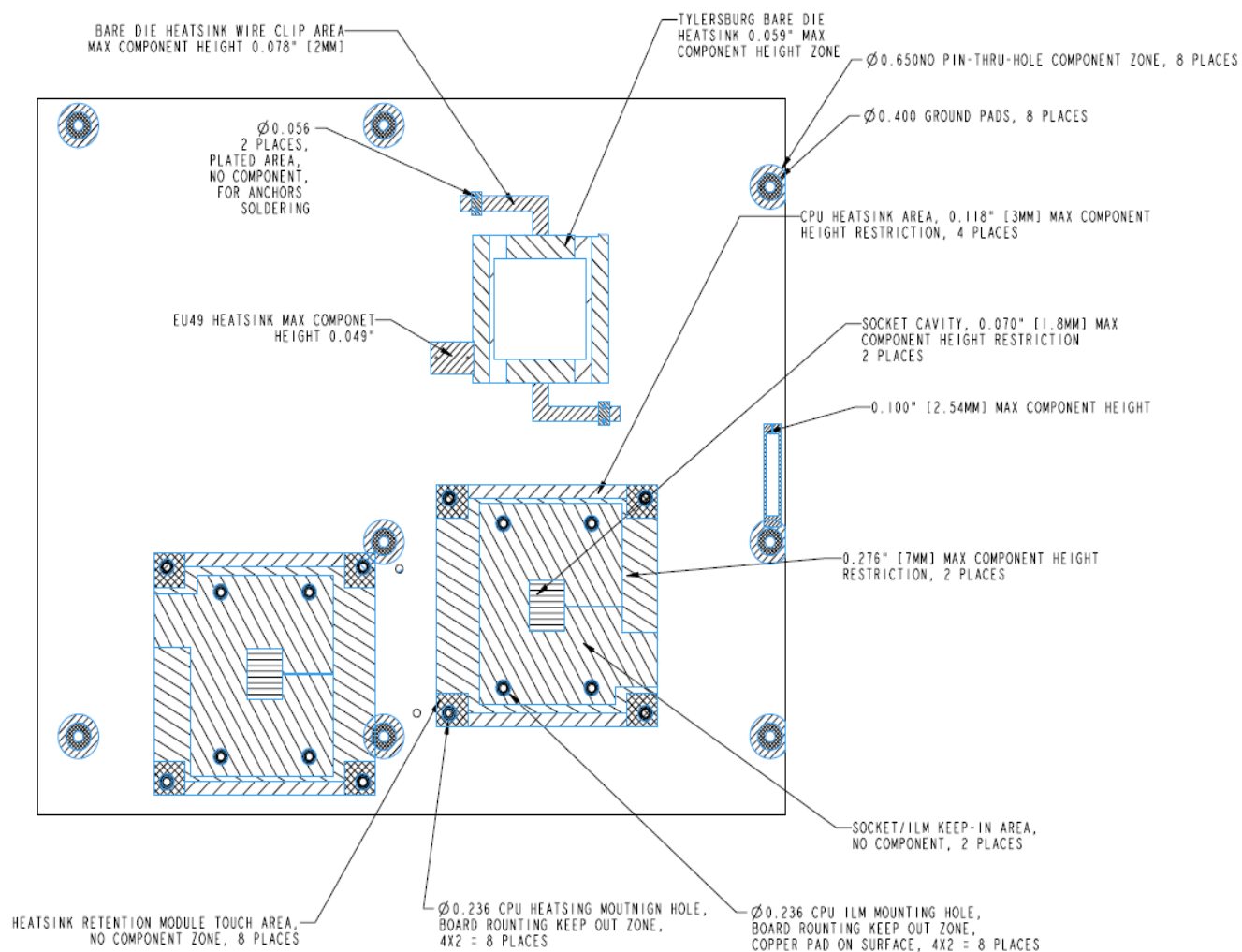
Figure 6. Intel® Server Board S5500BC Board Primary Side Keepouts
