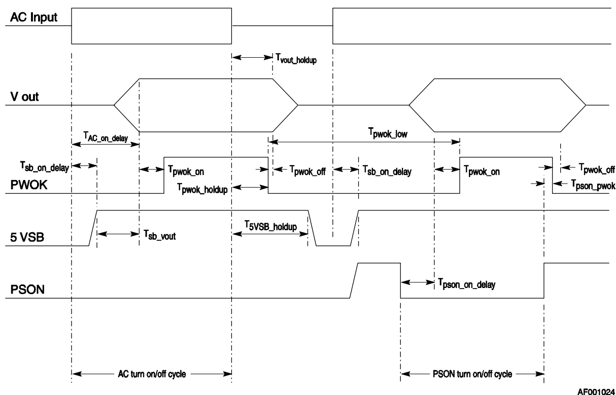
Figure 47. Turn On/Off Timing (Power Supply Signals)
